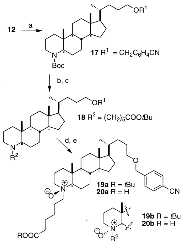
Scheme 4. Conditions: (a) 4-NC-C 6 H 4 CH 2 Br, NaH, 91%; (b) TFA, CH 2 Cl 2 , 1 h; (c) Br(CH 2 ) 5 COOtBu, NEt 3 Pr 2 , DMF, 60 °C, 40 h, 57%; (d) m CPBA, CH 2 Cl 2 , -20 °C → rt, 4 h, 99%, separation of epimers; (e) TFA, CH 2 Cl 2 , 4 h, 99%.
