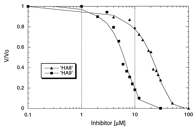
Figure 1. Dose-response plot of inhibition by 1a (HA8) and 1b (HA9). Conditions: 5 \mu M IgG HA8-25A10; 400 \mu M substrate 2 ; 0.2% TWEEN 80; 50 mM phosphate buffer; pH 7.0; 37 °C. IC_{50} values derived from plots: 18.9 \mu M ( 1a ), 5.7 \mu M ( 1b ).
