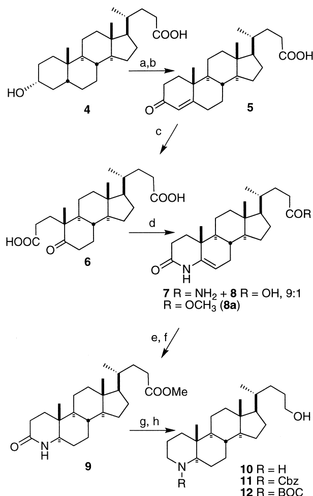
Scheme 2. Conditions: (a) NBS, dioxane/H 2 O; (b) Li 2 CO 3 , DMF, 90 °C; (c) KMnO 4 , NaIO 4 , t BuOH reflux, 89%; (d) liquid NH 3 , HOCH 2 CH 2 OH, 5–180 °C, 83%; (e) 600 p.s.i. (40 bar H 2 , 10% Pd/C, glacial HOAc, PARR BOMB, 5 d; (f) amberlyst 15, MeOH, reflux, 75% over 2 steps; (g) LiAlH 4 ; (h) CbzCl ( 9 → 11 ), 60–68% over 2 steps.
