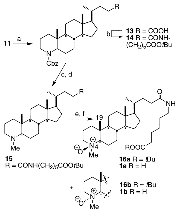
Scheme 3. Conditions: (a) pyridinium dichromate, 71%; (b) H 2 N(CH 2 ) 5 COO t Bu, EDC, NEt 3 , DMF, 91%; (c) H 2 , 10% Pd/C; (d) 40% formalin, NaBH 4 , 25 °C, 70% over 2 steps; (e) m CPBA, 61% separation of epimers; (f) TFA, 84%.
